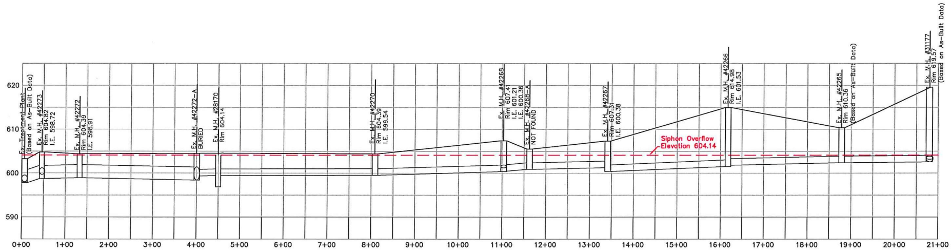
PROFILE #2 - JTOWN RELIEF INTERCEPTOR
